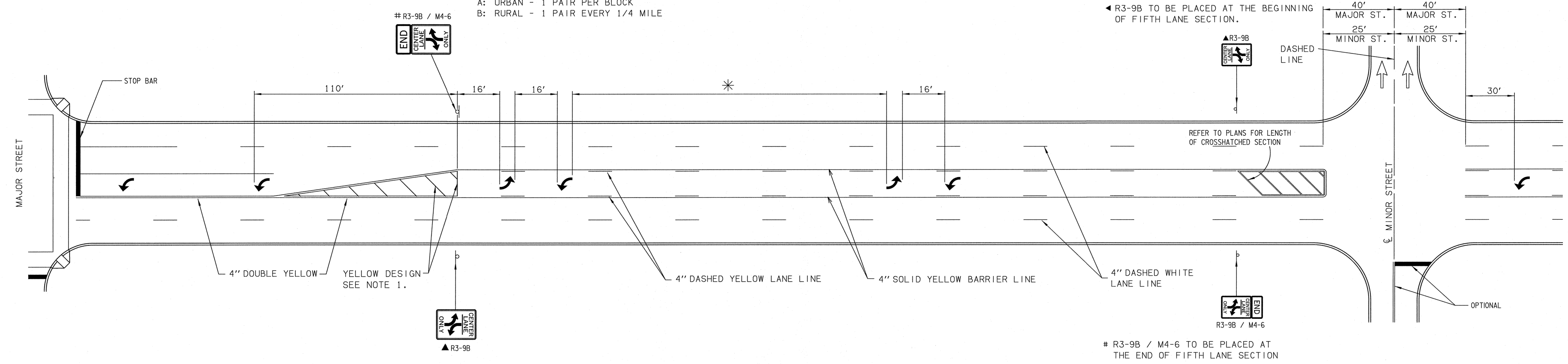
FIFTH LANE PAVEMENT MARKING DETAIL (URBAN)
