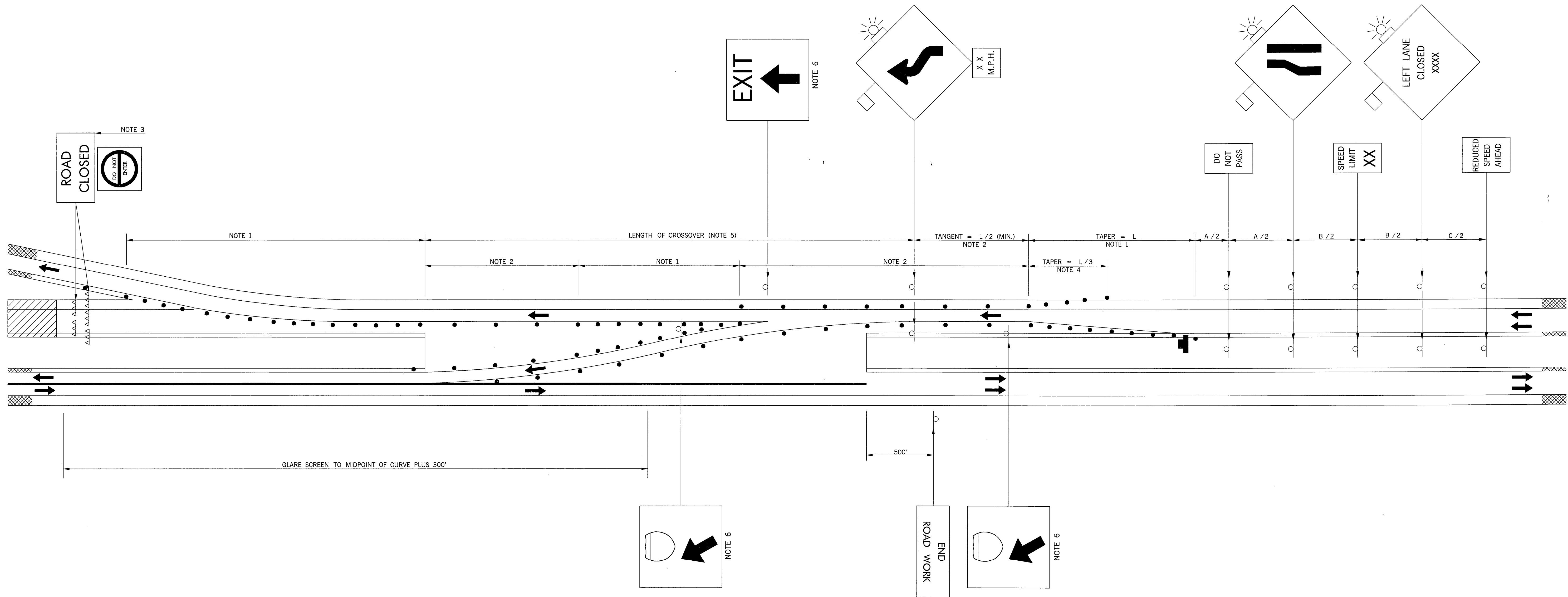
TYPICAL APPLICATION CROSS-OVER, WITH RAMP ACCESS (ONE SIDE)
