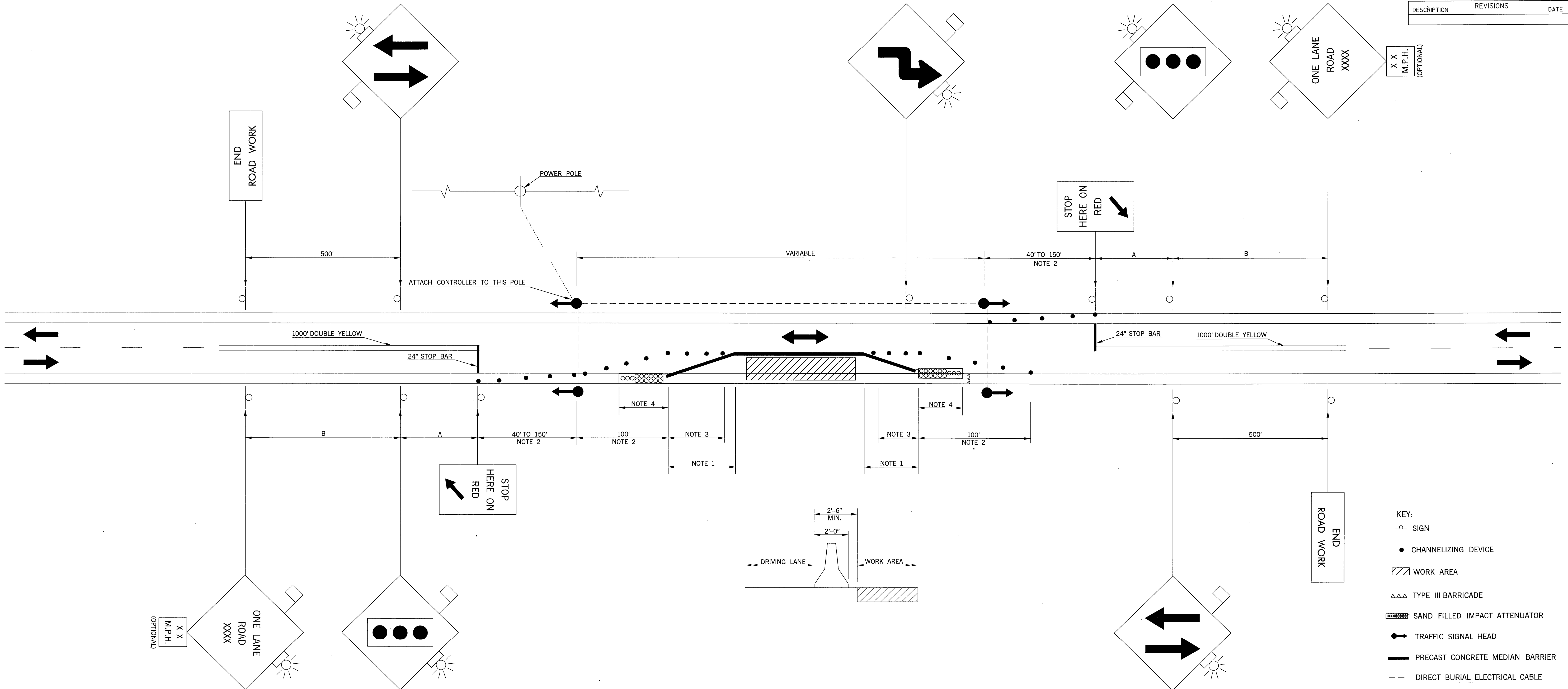
TYPICAL APPLICATION – USING TRAFFIC SIGNALS AND MEDIAN BARRIER
