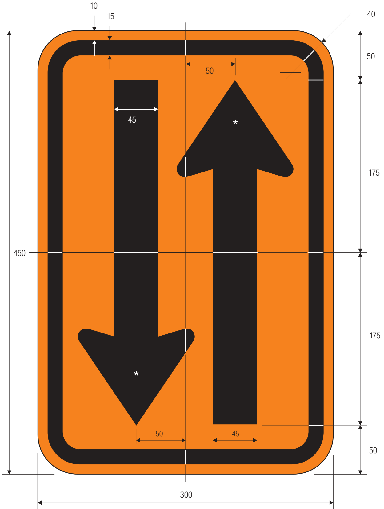
W6-4
