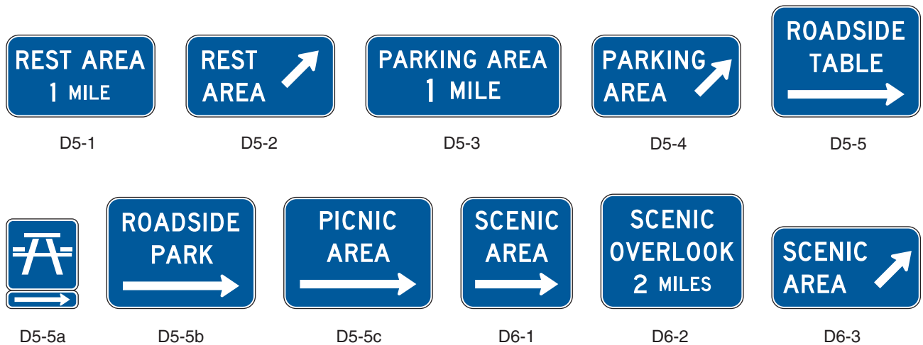
Figure 2D-9. Rest Area and Scenic Overlook Signs
