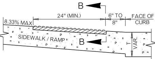
SECTION X - X TYPE B DOMED TILE SYSTEM (WET SET INLAY)
