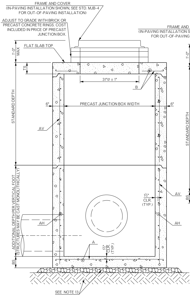
SECTION A-A - STANDARD DEPTH
