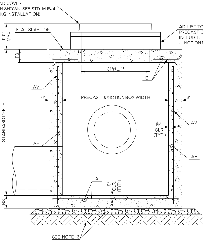
SECTION A-A - NON-STANDARD DEPTH
