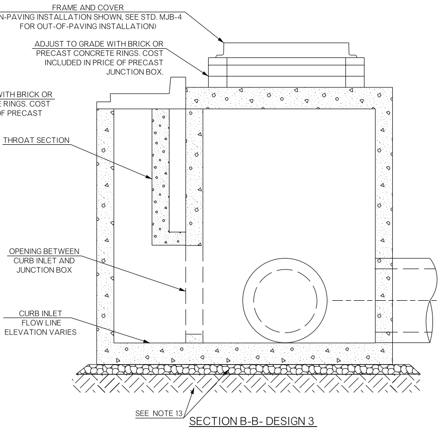
SECTION B-B - DESIGN 3
