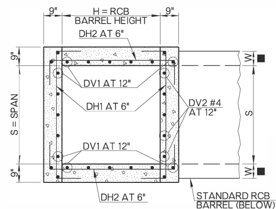
SECTION B-B THRU INLET
