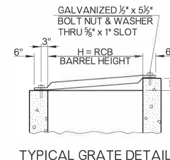
TYPICAL GRATE DETAIL
