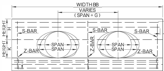
END VIEW (PIPE GRATES NOT SHOWN THIS VIEW)
