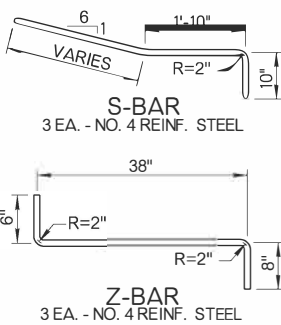
S-BAR 3 EA. - NO. 4 REINF. STEEL
