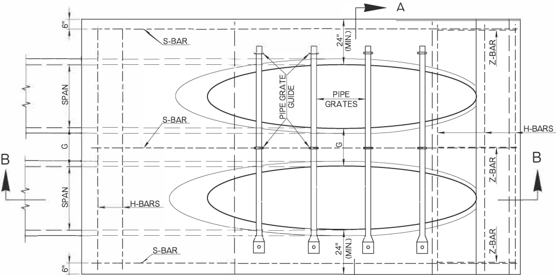
PLAN (SIDE DRAIN SHOWN)
