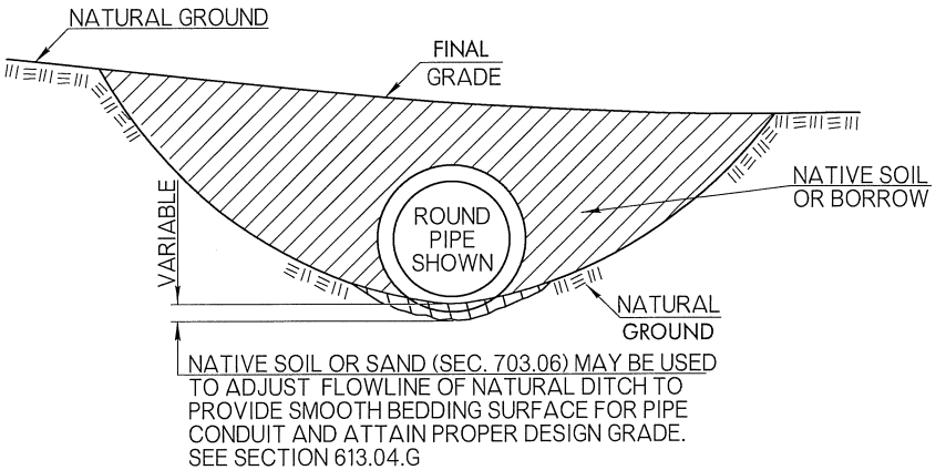
CLASS D BEDDING ALTERNATE 2
