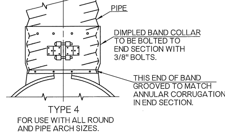
TYPICAL METAL END SECTION CONNECTIONS
