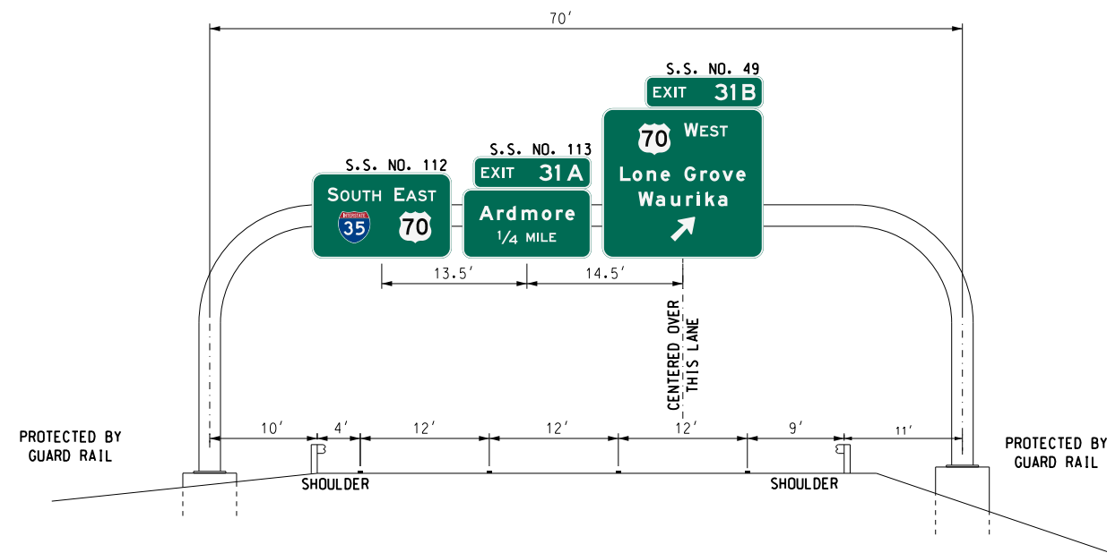
SIGN STRUCTURE NO. 6 70' TYPE "B" MONOTUBE I-35 SOUTH BOUND APPROX. MILE MARKER 31+5250 (458.0 S.F.)
