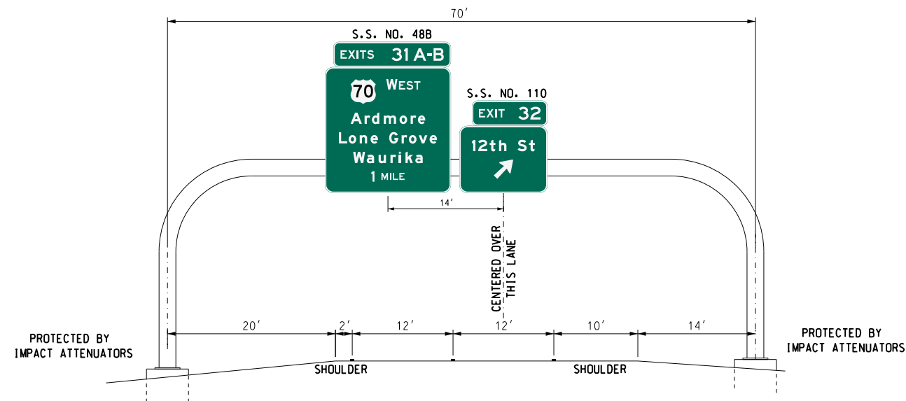
SIGN STRUCTURE NO. 5 70' TYPE "B" MONOTUBE I-35 SOUTH BOUND APPROX. MILE MARKER 33+730 (378.0 S.F.)
