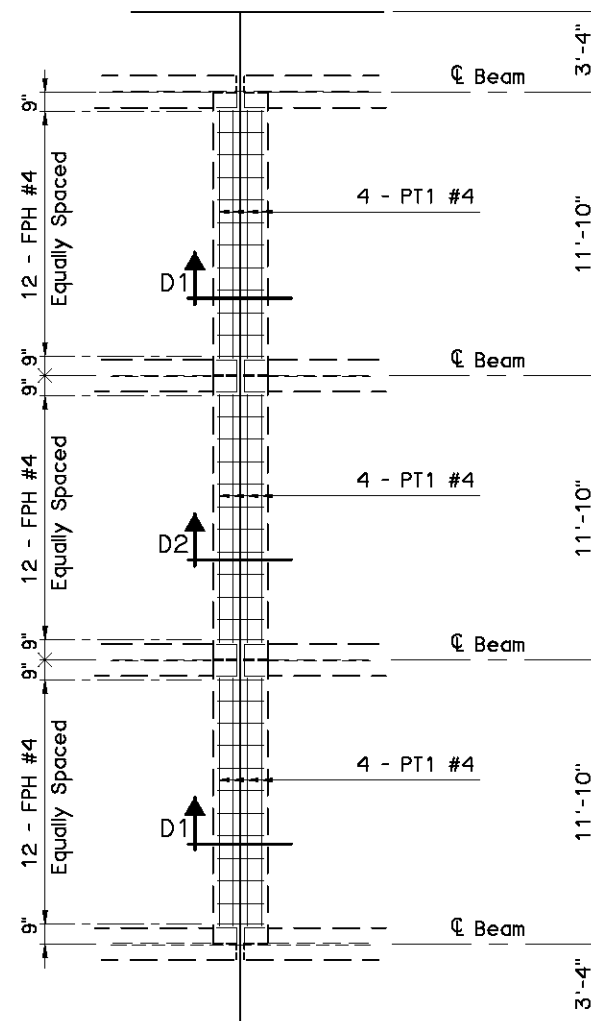
FIXED PIER
