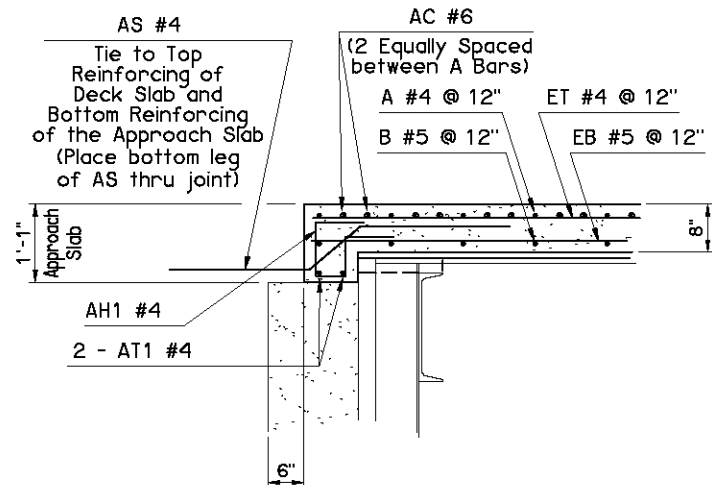
SECTION A
