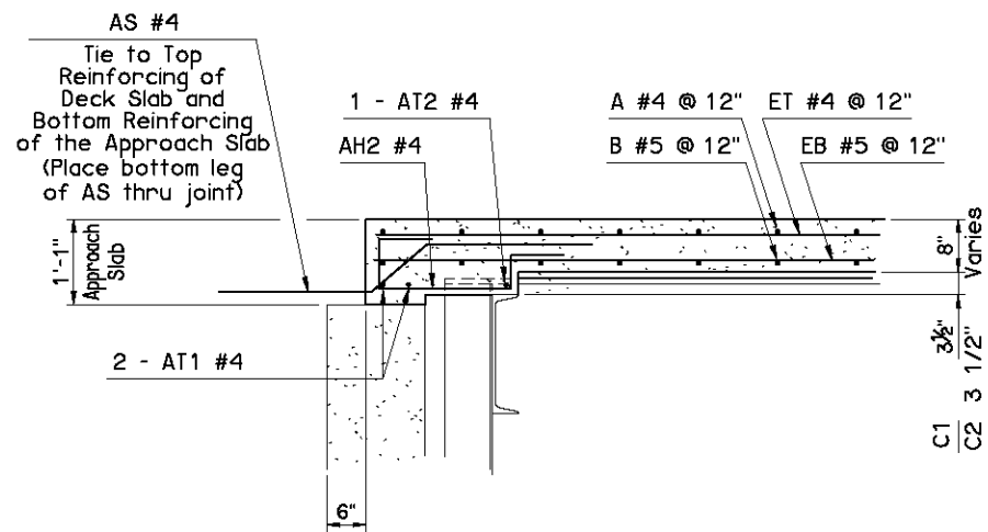
SECTION C1 AND C2
