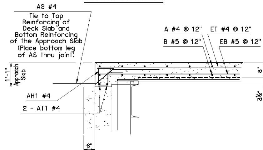
SECTION B
