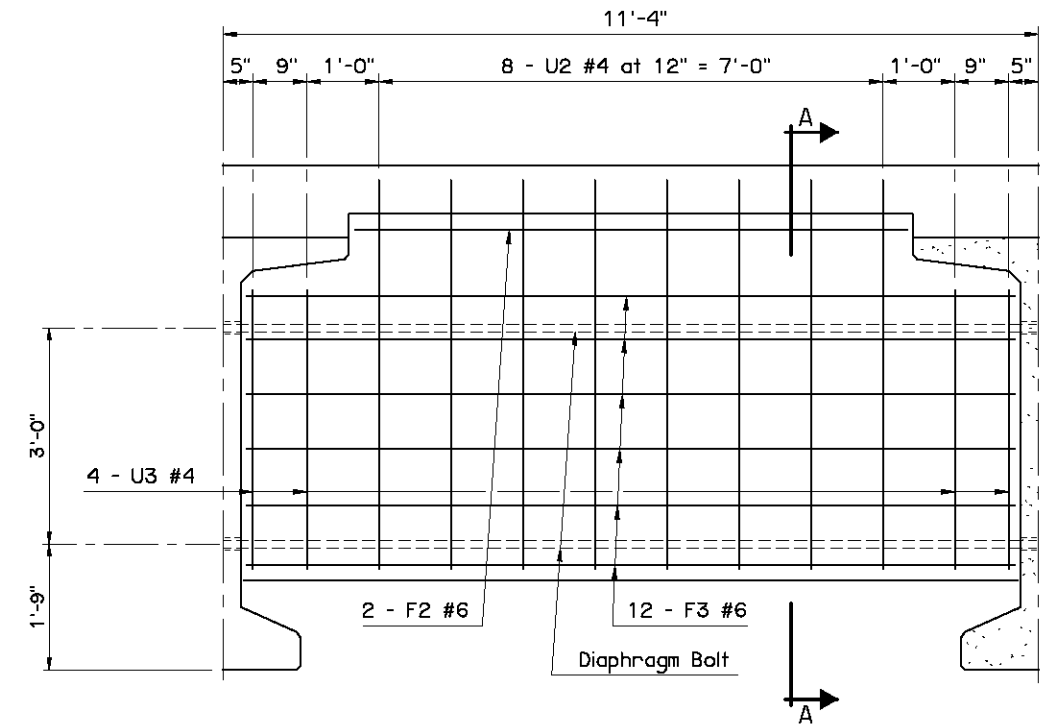
END DIAPHRAGM
