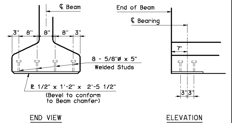
EMBEDDED SOLE PLATE DETAILS
