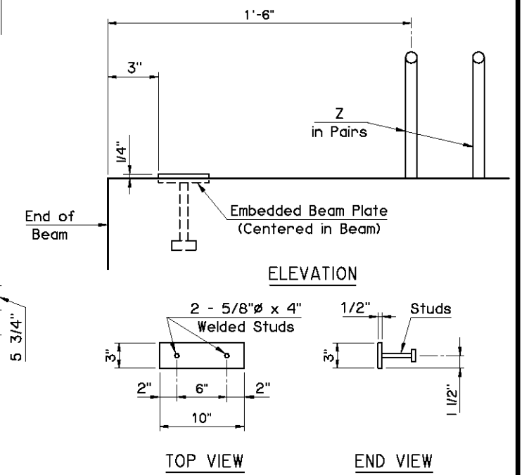
EMBEDDED BEAM PLATE DETAILS
