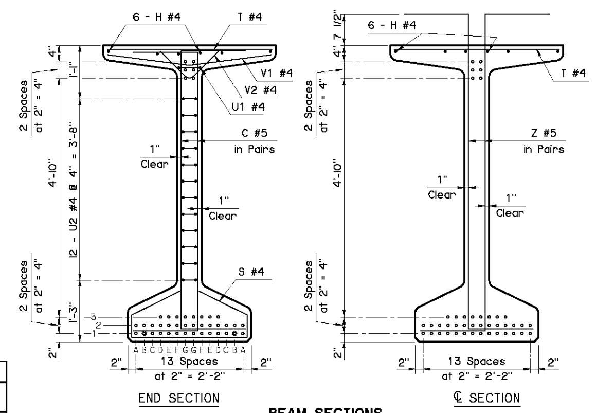
BEAM SECTIONS (42 - 0.6" STRANDS)
