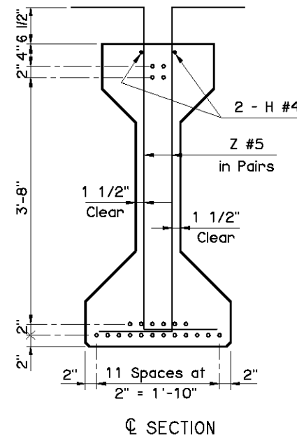
BEAM SECTIONS (22 - 0.6"Ø STRANDS)
