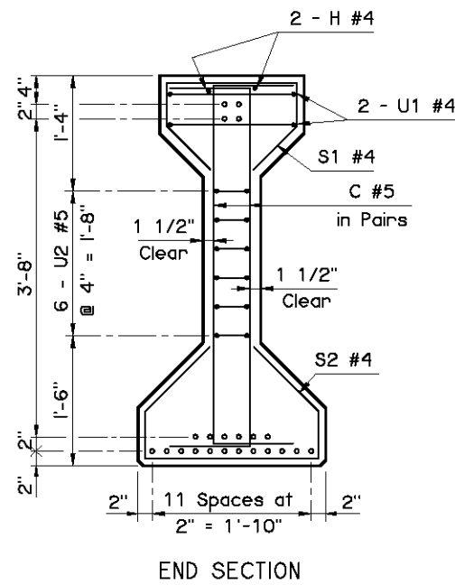
BEAM SECTIONS (22 - 0.6"Ø STRANDS)
