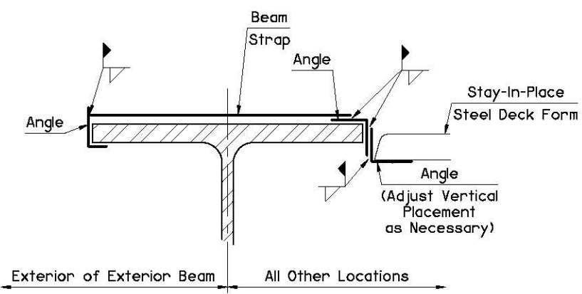
STAY-IN-PLACE STEEL DECK FORM FLANGE CONNECTION DETAIL
