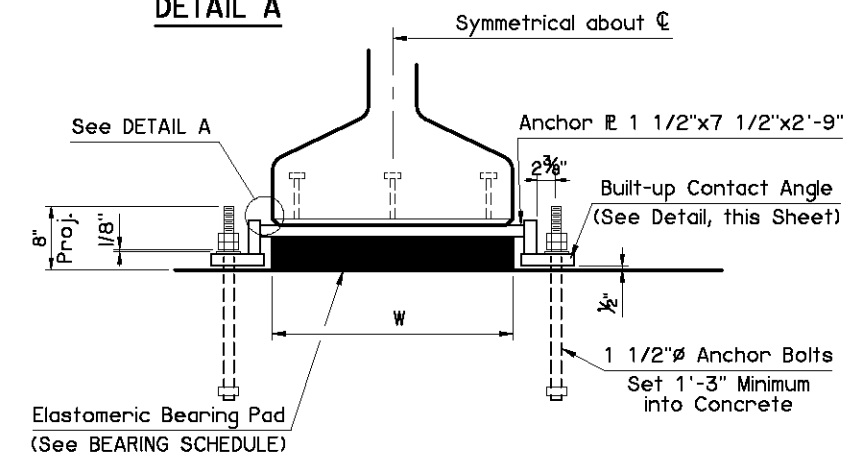
PIER EXPANSION BEARING DETAILS
