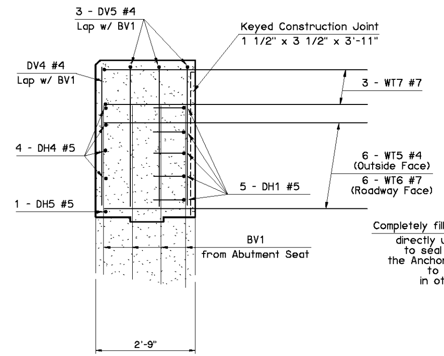
SECTION C-C
