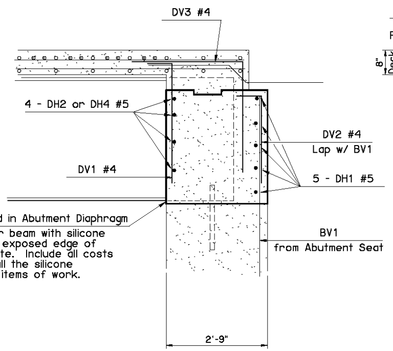
SECTION B-B
