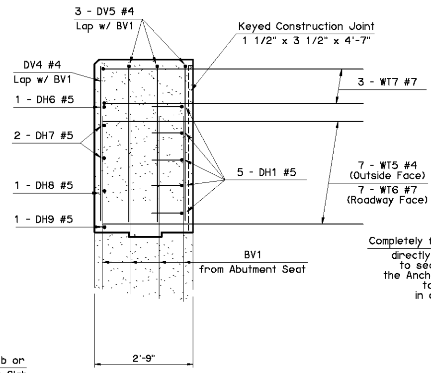
SECTION C-C
