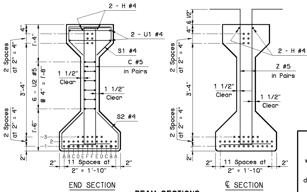
BEAM SECTIONS (36 - 0.6"Ø STRANDS)
