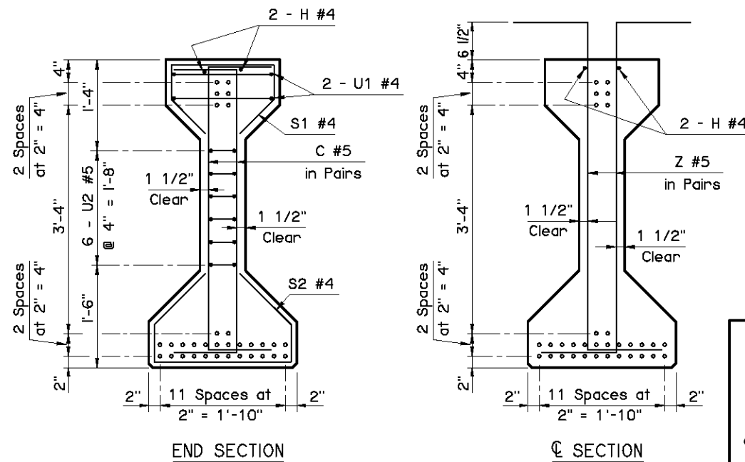
BEAM SECTIONS (32 - 0.6" STRANDS)
