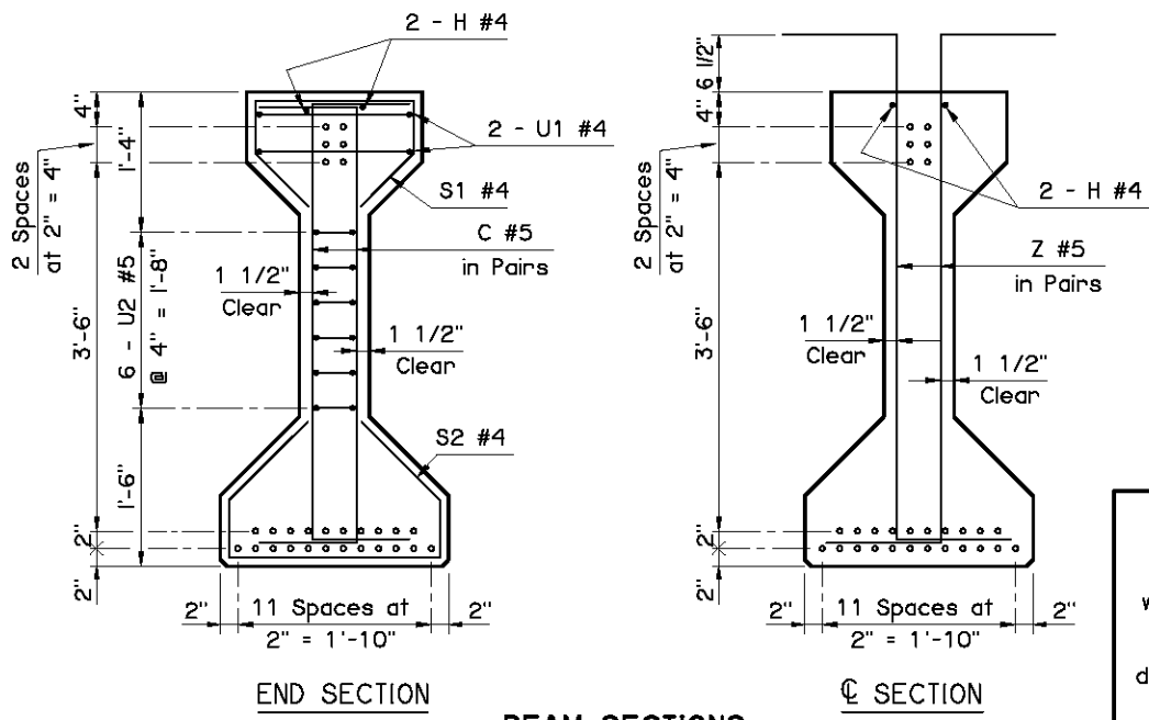
BEAM SECTIONS (28 - 0.6"Ø STRANDS)
