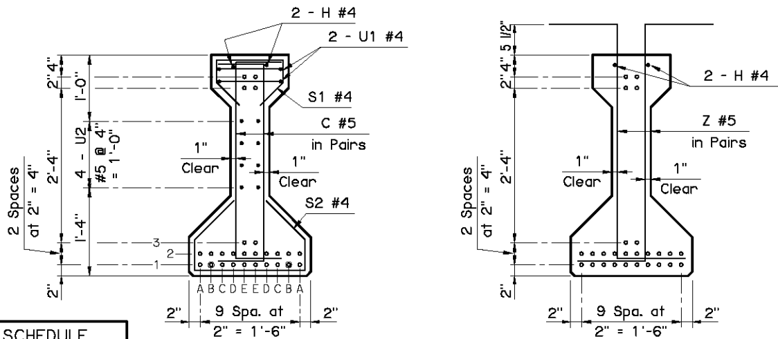
BEAM SECTIONS (26 - 0.6" STRANDS)
