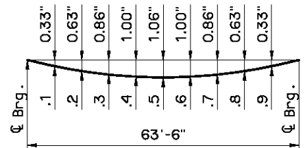
DEAD LOAD DEFLECTION DIAGRAM
