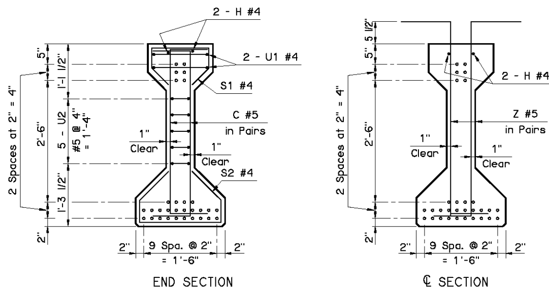
BEAM SECTIONS
