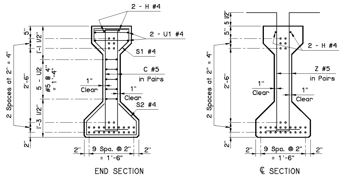
BEAM SECTIONS (28 - 0.6" STRANDS)
