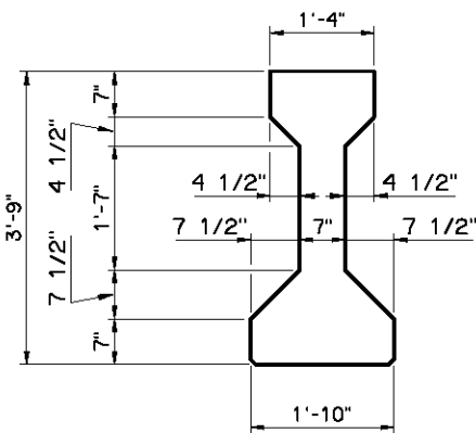
END VIEW (Type III P.C.B.)
