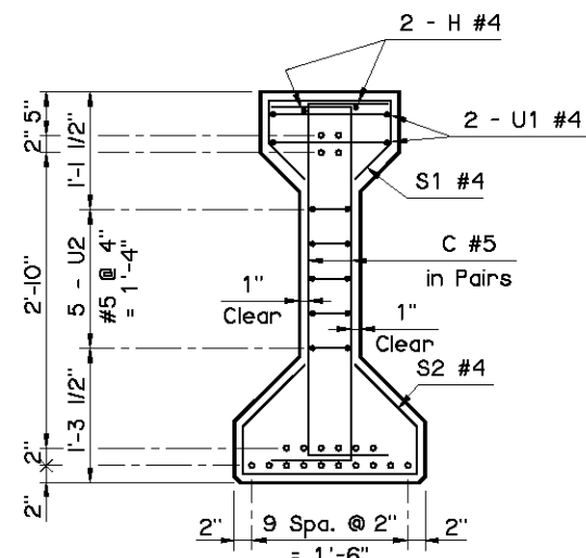
END SECTION
