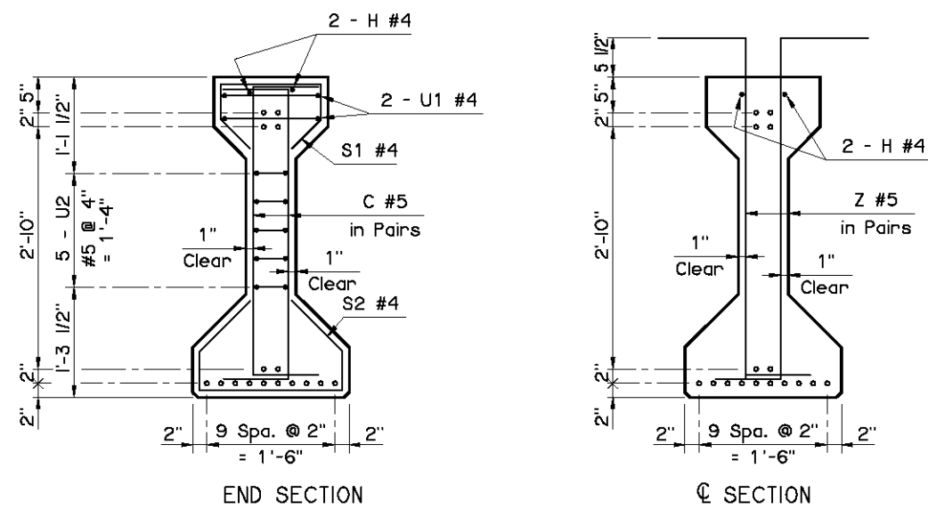
BEAM SECTIONS (16 - 0.6" STRANDS)
