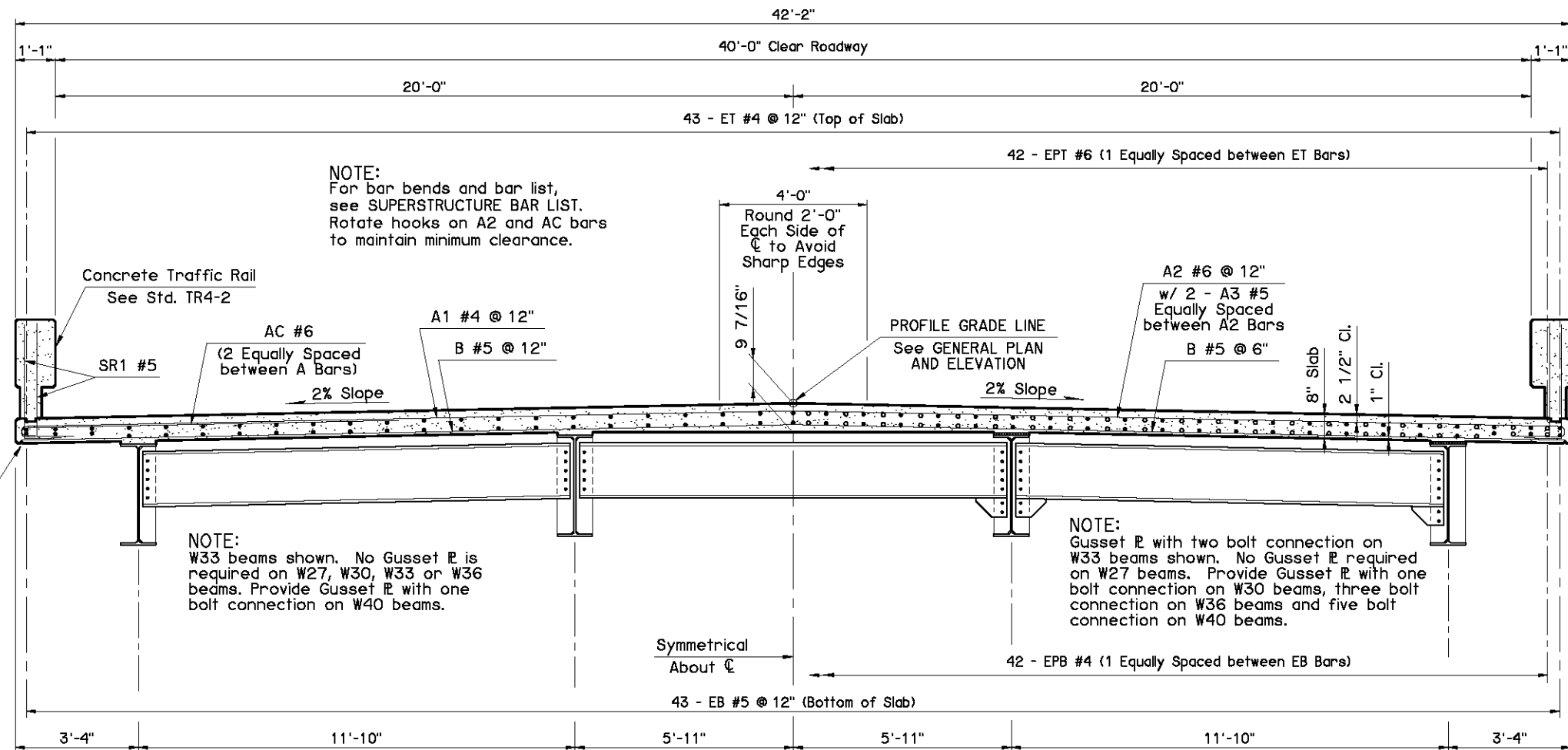
HALF SECTION AT INTERMEDIATE DIAPHRAGM
