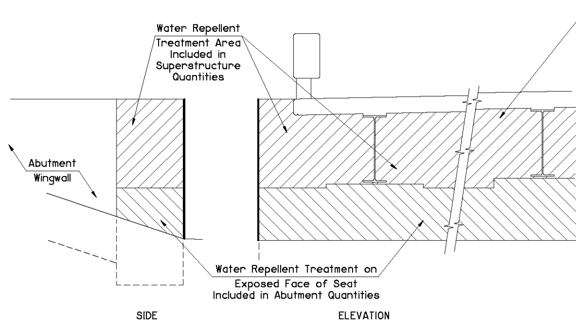
ABUTMENT DIAPHRAGM
