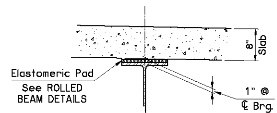
BEAM HAUNCH DETAIL
