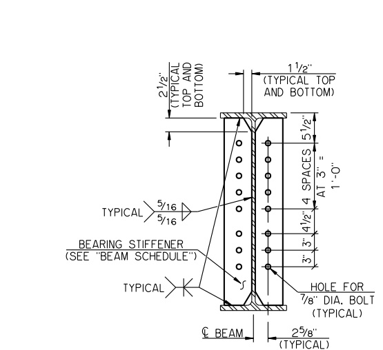
SHEAR CONNECTOR DETAIL
