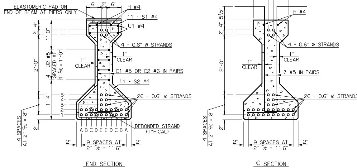
BEAM SECTIONS (30 - 0.6" Ø STRANDS)
