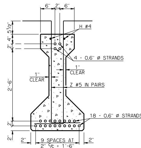
CL SECTION
