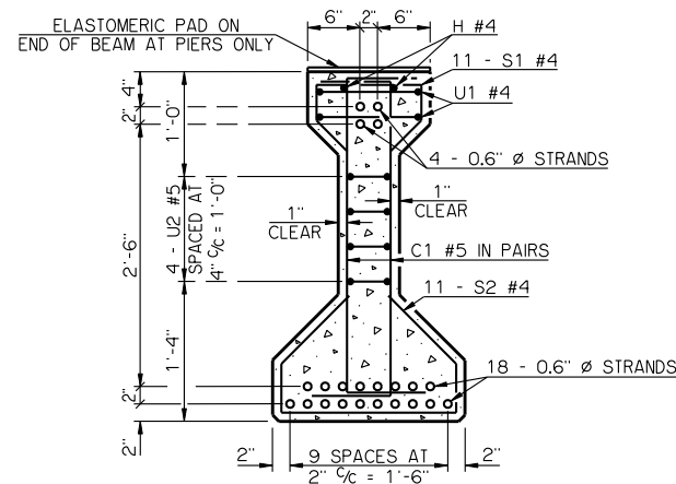
END SECTION
