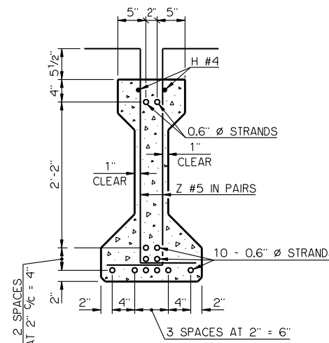
CL SECTION
