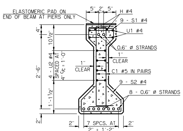
END SECTION
