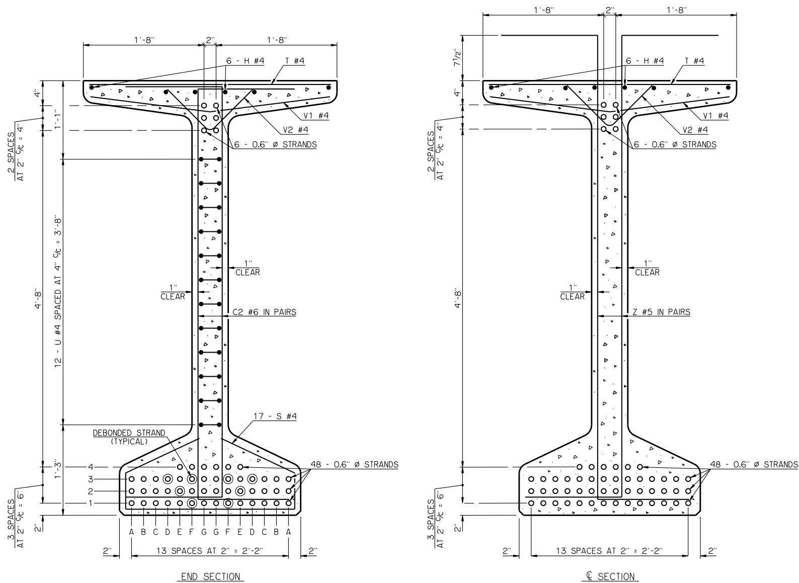
BEAM SECTIONS (54 - 0.6" Ø STRANDS)
