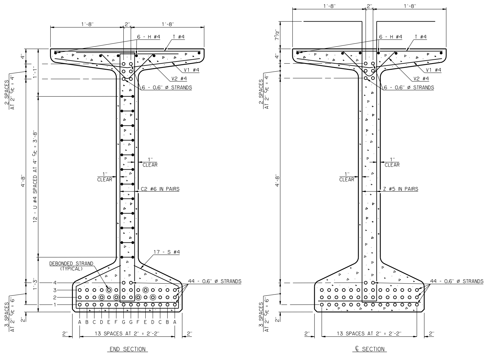
BEAM SECTIONS (50 - 0.6" Ø STRANDS)
