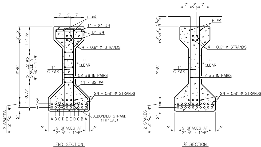
BEAM SECTIONS (28 - 0.6" Ø STRANDS)
