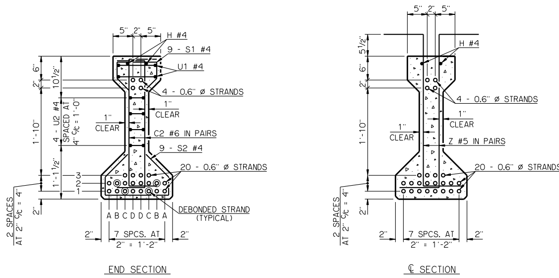
BEAM SECTIONS (24 - 0.6" \phi STRANDS)
