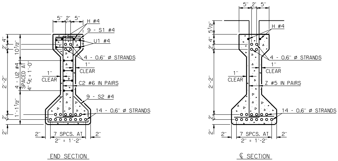
BEAM SECTIONS (18 - 0.6" \phi STRANDS)
