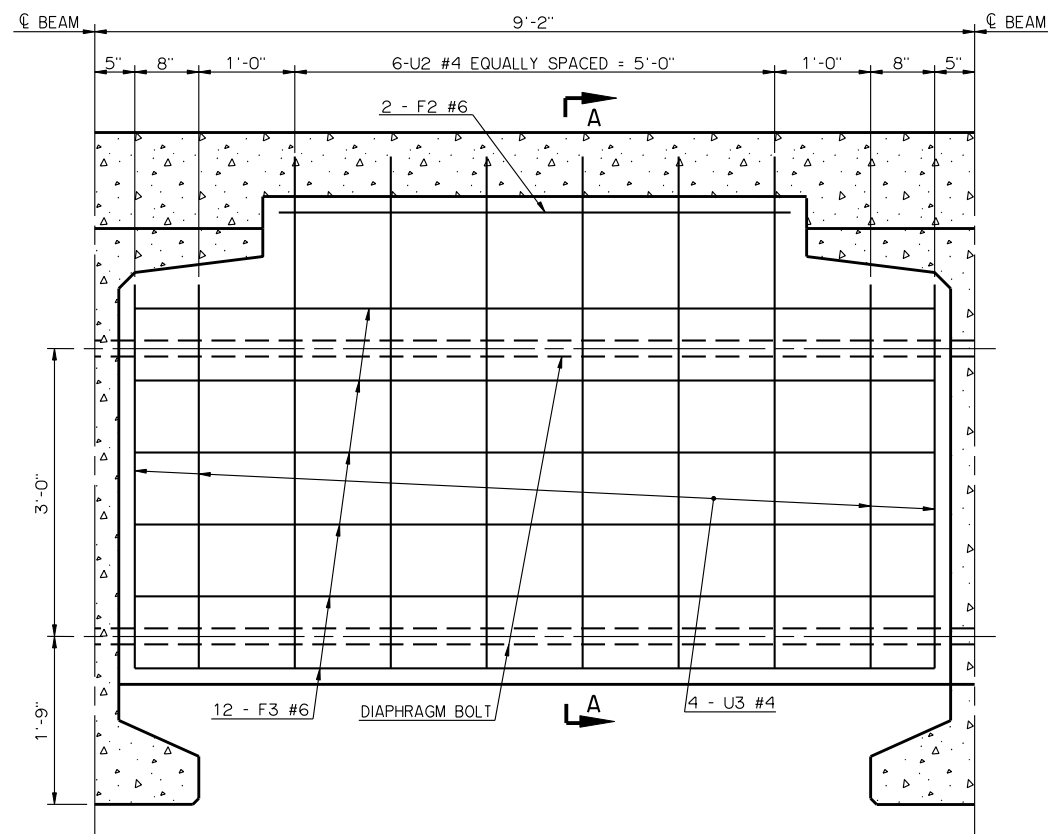
END DIAPHRAGM ELEVATION
