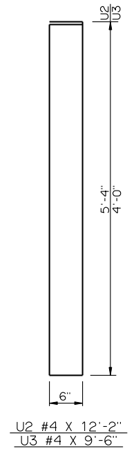
DETAILS OF BENT REINFORCING STEEL
