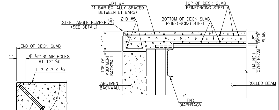
TYPICAL SLAB REINFORCING AT ABUTMENT BACKWALL
