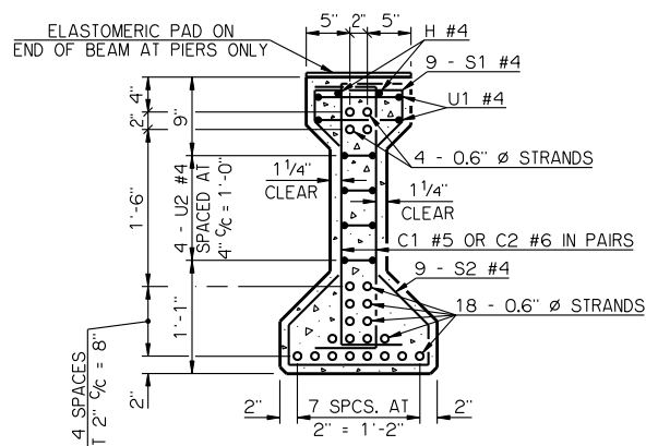
END SECTION
