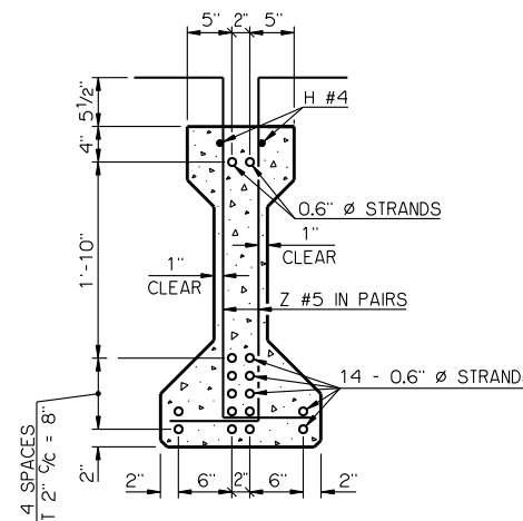
CL SECTION
