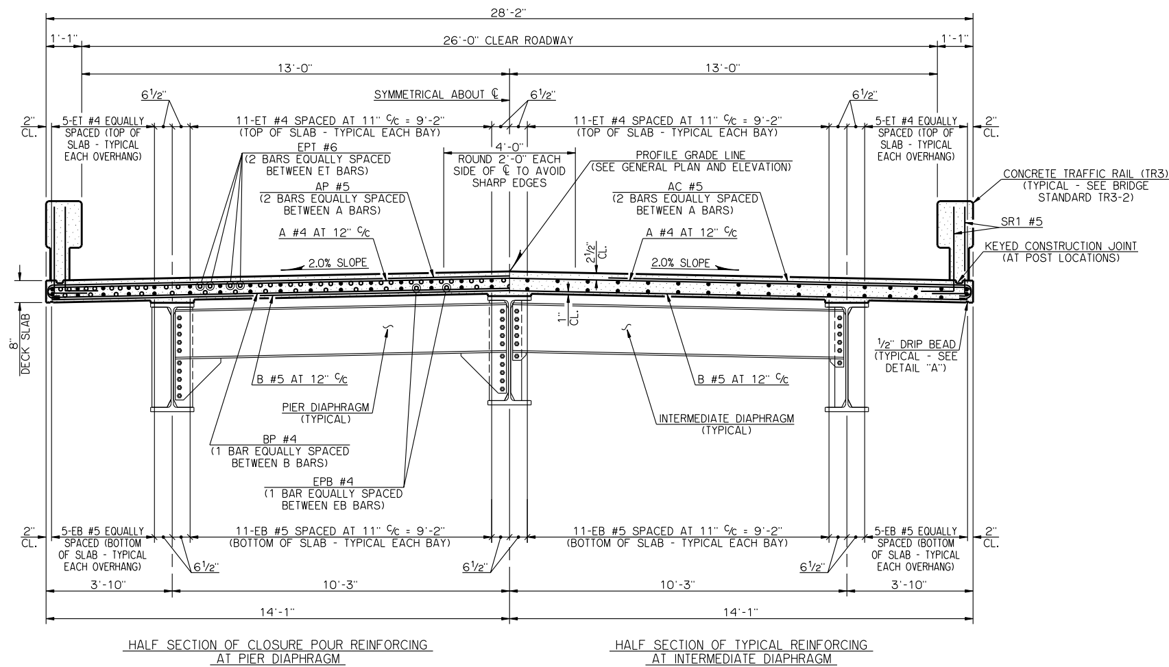
TYPICAL CROSS SECTION
