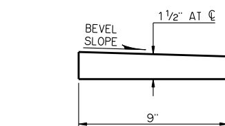
BEVELED ANCHOR PLATE DETAIL
