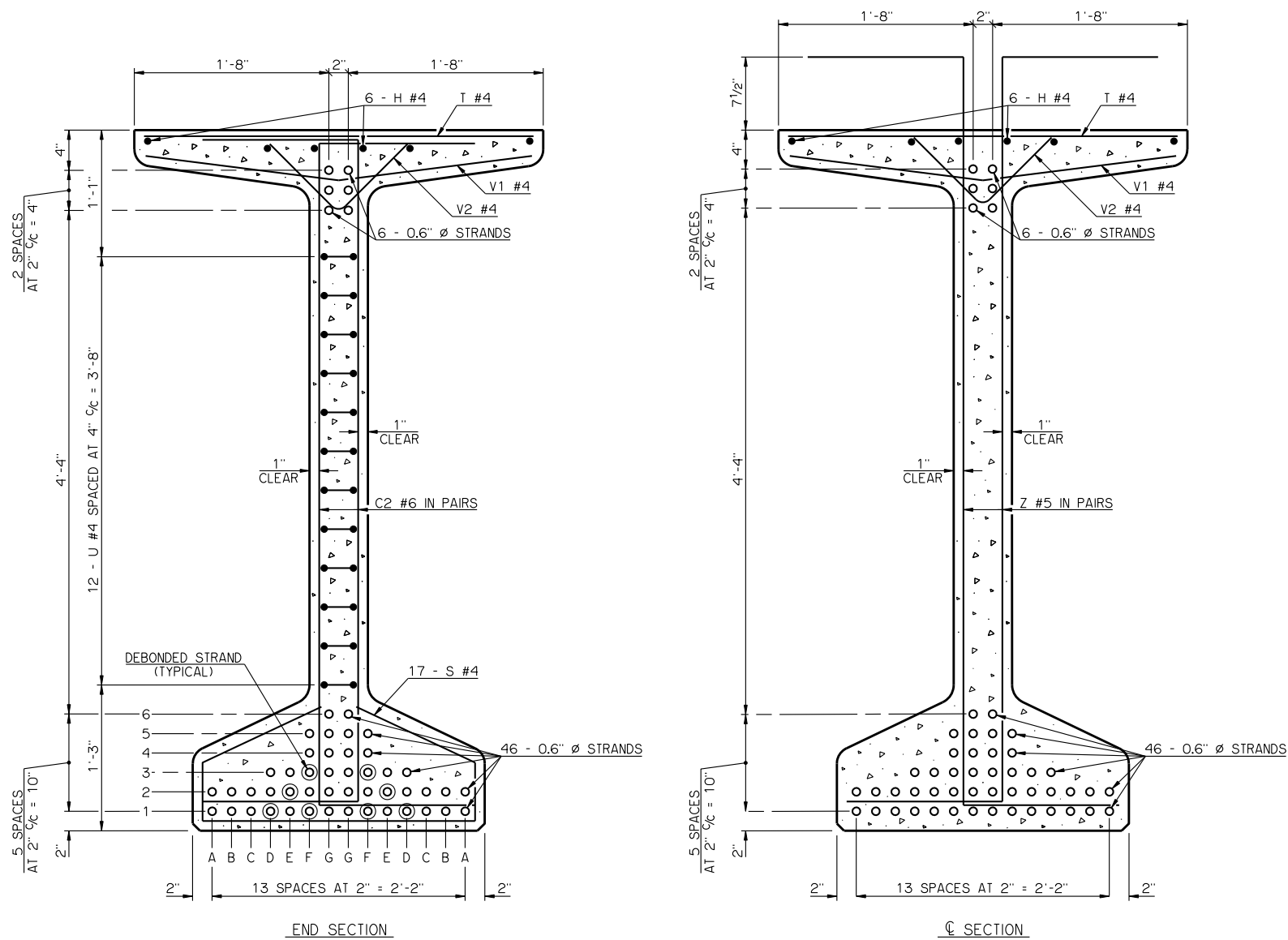
BEAM SECTIONS (52 - 0.6" Ø STRANDS)
