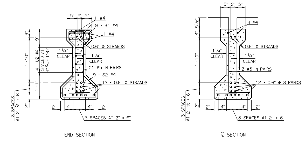
BEAM SECTIONS (14 - 0.6" \phi STRANDS)
