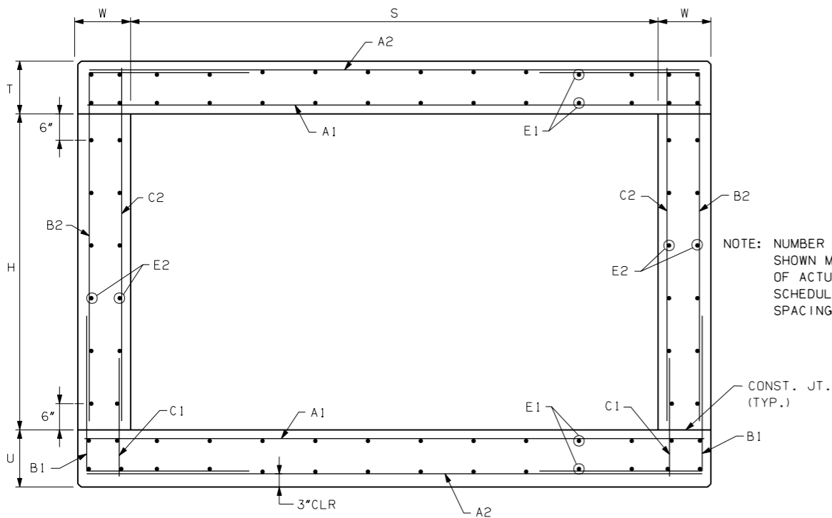
BARREL SECTION
