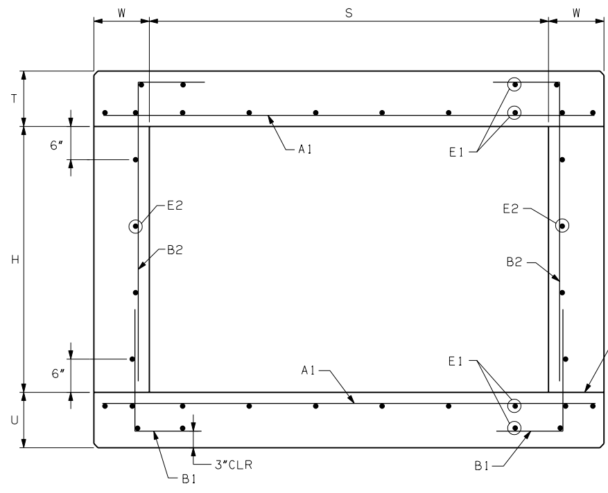
BARREL SECTION
