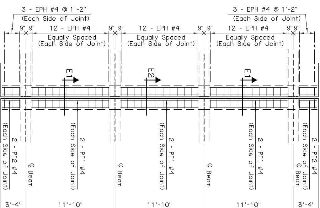
EXPANSION PIER
