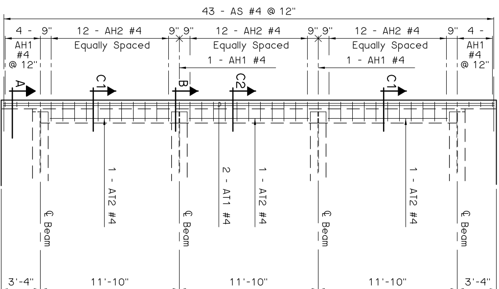
ABUTMENT
